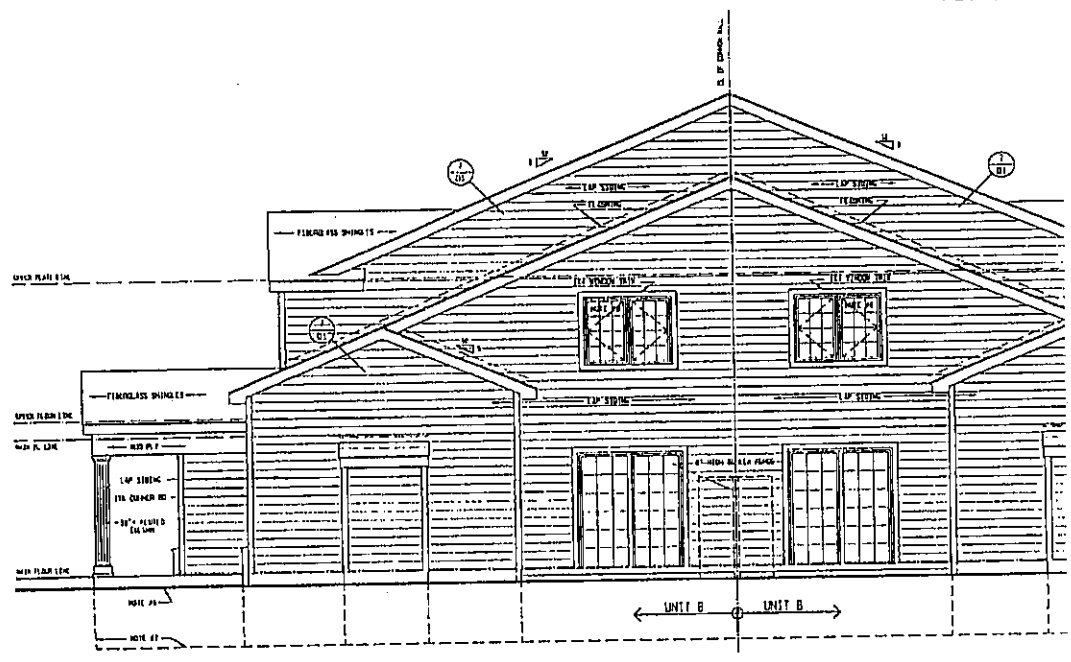
RIGHT/LEFT ELEVATION SCALE 1/4" = 1'-0"
