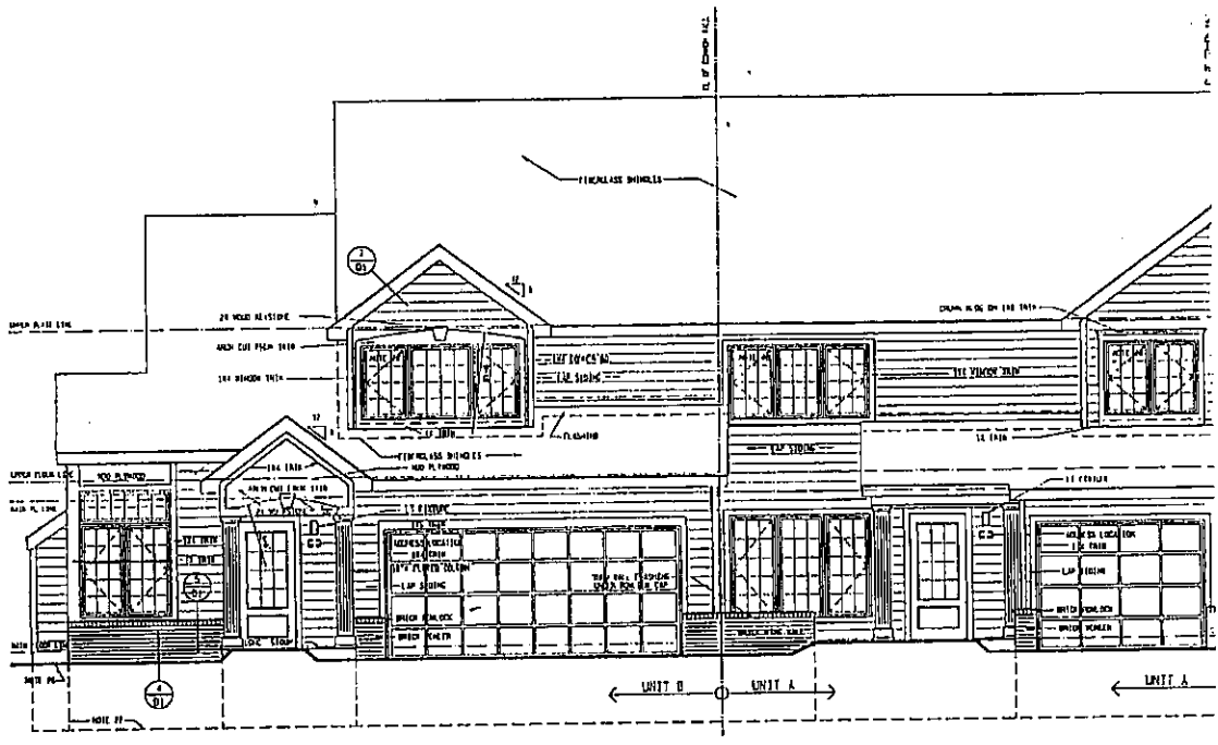
FRONT/REAR SCALE 1/4" = 1'-0"
